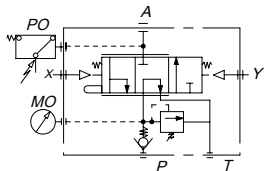
HYDRAULIC SYMBOL
